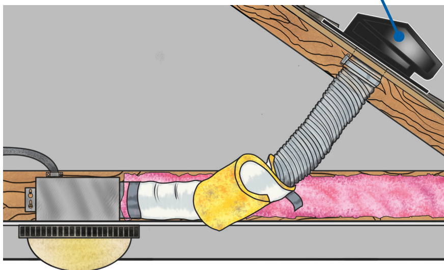
Example installation of BATH PRO for a bathroom exhaust fan
